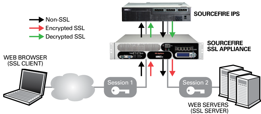
Figure 2. Inline IPS Configuration
